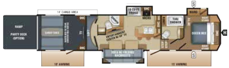
SEISMIC | 4114 | OPTION B Ext. Lgth: 44' 11" Ext. Ht: 161" Unloaded Wt. (lbs): 15,310 Sleeps: 7-8
